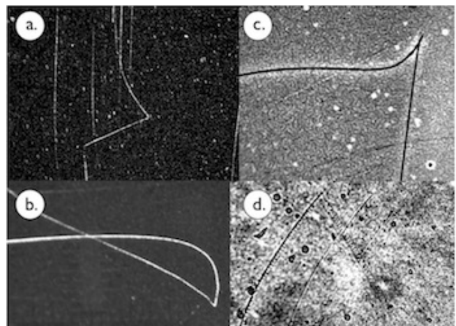
FIG. 26. a.) One of a series of tracks with progressive curvature. Concave reversed track. Exact fit to parabola b.) The classic vertex form. Convex positive track. Exact fit to parabola c.) The concave form of the vertex. Reversed track. Exact fit to parabola d.) Small convex form track using 400x magnification. Evaporated track. Exact fit to parabola.
