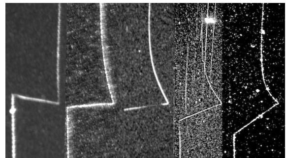
FIG. 23. Progressive curvature seen in a correlated group of tracks from the same exposure.
