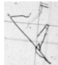
FIG. 18. Ivoilov "chiral" tracks where right track was flipped horizontally and vertically and overlaid on left track. Note correspondence on main track and misalignment on other tracks. Compare with Fredericks tracks in Fig. 16 where 2 correlated tracks are overlaid.
