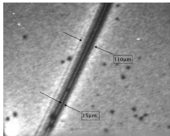
FIG. 25. Sub Tracks Detail Micrograph at 45x magnification showing sub-track structure of the track bundle.
