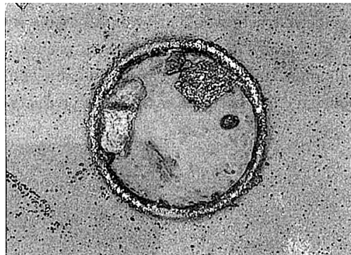
FIG. 35. Ring track of Matsumoto
