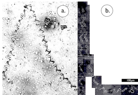
FIG. 4. a.) Fredericks track b.) Adamenko and Vysotskii track evaporated in MDS showing parabolic curvature. Detail of track using high magnification.
