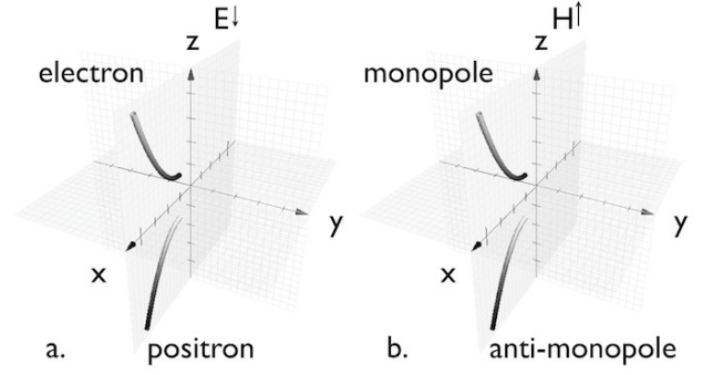
FIG. 27. a.) An electric field, E is applied along the z -axis in the -z direction. Due to the E field, electrons curve upward and positrons curve downward in a parabola in the x, z plane. b.) A magnetic field, H is applied along the z -axis in the +z direction. Due to the H field, magnetic monopoles curve upward and anti-monopoles curve downward in the x, z plane.
