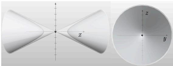
FIG. 34. Top and end views of tachyon shape.
