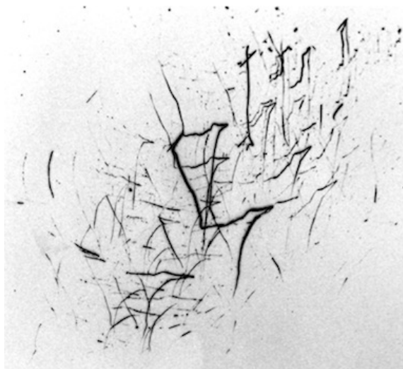
FIG. 24. Vector Swarm Group correlation of tracks including random motion components. These tracks do not line up when overlaid. They change form with location, apparently due to relative position in the applied non-uniform magnetic field. A large number of the tracks in this exposure are correlated. A measure of corresponding line segments of matching groups of tracks reveals a macroscopic “central force,” which will be the subject of future work.
