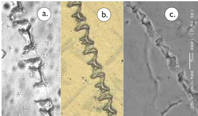
FIG. 3. a.) Fredericks track on Polychrome litho film. b.) Rodionov and Savvatimova periodic structure track on nuclear emulsion. Note similarity to Fredericks track where "hour-glass" structures are separated by flat structures. c.) Rodionov and Savvatimova periodic structure track on Pd cathode from scanning electron microscope.
