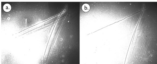
FIG. 20. Matsumoto correlated tracks overlaid. The shape of the image and certain ring positions correspond.
