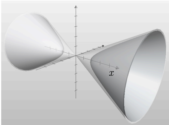
FIG. 33. Shape of tachyon (between conic and hyperbolic surfaces) with motion in x direction after an SLT as a subluminal observer in frame f would see it.
