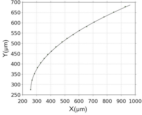
FIG. 29. Track 4. bobby pins fit to general quadratic eq. (2).
