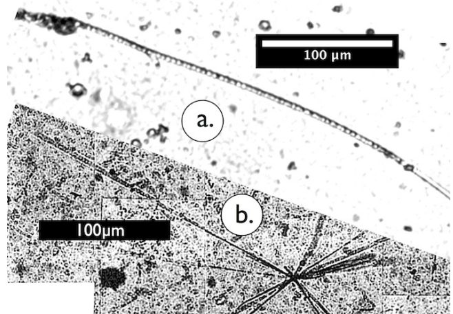
FIG. 7. Both tracks exhibit regular periodic "circles" in tracks. a.) Fredericks track b.) Matsumoto star in Fujifilm MA-7B nuclear emulsion.
