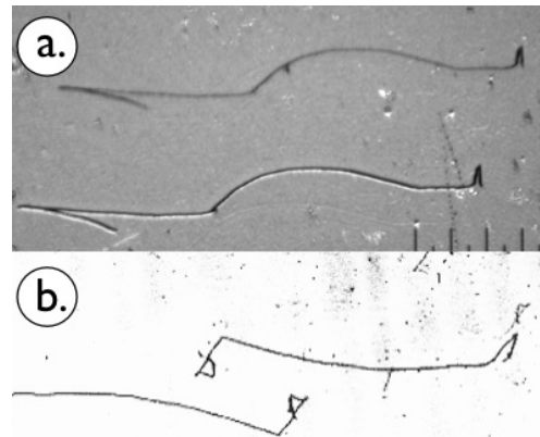
FIG. 2. a.) Fredericks tracks. Correlated tracks in Kodak Kodalith type III film. Tracks are copies instead of mirror images or chirally transformed. b.) Ivoilov “chiral” tracks. Multiple correlated tracks can be seen in the original image. The chirally transformed track is explained in the Ivoilov analysis as a reflected track which is recorded on the bottom emulsion facing an aluminum plate with polyester base material sandwiched between the two emulsion layers. Unspecified type of double-sided X-ray emulsion.
