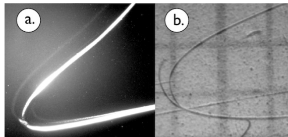
FIG. 5. a.) Fredericks track. b.) Priem, et.al. track. On both tracks, parabolic curvature and splitting are seen.
