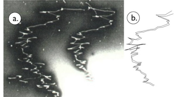
FIG. 16. a.) Correlated random motion trajectories. Kodak 10 \mu NTB3 emulsion. b.) Using a graphics editor, the tracks were traced from the original. The tracks when superimposed upon each other reveal very similar though not quite identical structure.
