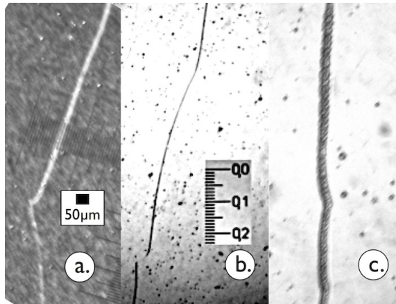
FIG. 6. a and b are classic 2-tailed vertexes with convex curvature. The curved part of track b is difficult to see, but appears to be parabolic. Track a was measured to be parabolic. a.) Fredericks track in Kodak Kodalith type III film. b.) Bardout, et al. track in Kodak Industrex MX125 (double-sided) film. c.) Related Lochak "laboratory" track[20] showing regular periodic structure.
