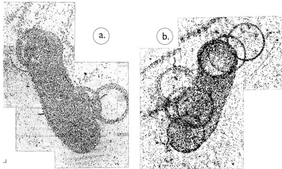
FIG. 19. Matsumoto correlated tracks as presented in original publication.
