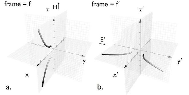
FIG. 32. a. Frame f where a magnetic field applied parallel to the z -axis is expected to cause parabolic curvature for magnetically charged bradyons in the x, z plane. b.) For tachyons , parabolic curvature occurs for electrically charged tachyons in the frame f' in the x', y' plane. For observables connected with electromagnetic fields, frame f' is related to frame f by a superluminal Lorentz transformation where \mathbf{H}_z = \mathbf{E}'_y .
