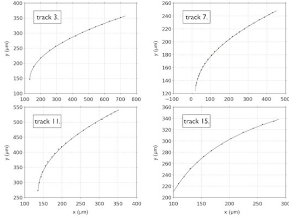
FIG. 30. Tracks 3, 7, 11 and 15 curve fits to general quadratic equations (2), (3) and (4) showing graphical fits to parabolas.
