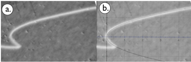
FIG. 14. hook , Curved track in Kodalith type III film. Applied magnetic field of permanent magnet M3. a.) raw track. b.) Graph of parabola x = y^2 overlaid on track
