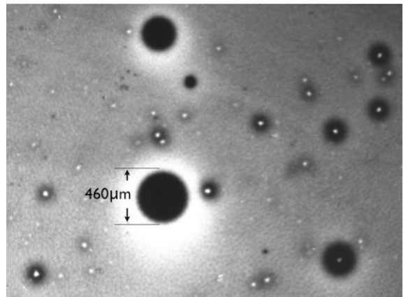
FIG. 9. Micrograph at 25x of dots. Note the internal structure of all-black dots and dots with white centers. Kodak type NTB3 10\ \mu emulsion.
