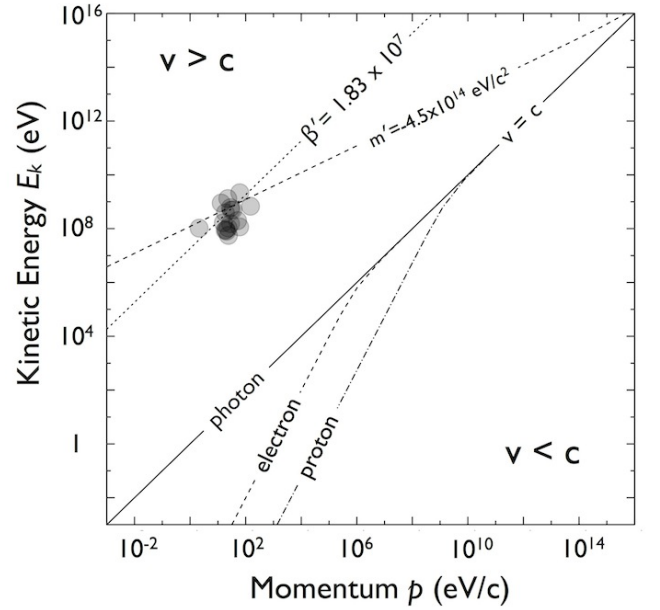
FIG. 31. A Recami-Mignani tachyon monopole with monopole charge, g = -e (in Gaussian units). Measured values for momentum and kinetic energy are clustered in the faster-than-light ( v > c ) area of the graph with a mass contour line computed with eq. (17) intersecting the peak mass value of |m| = 4.5 \times 10^5 \text{ GeV}/c^2 . The velocity contour line intersects the SLT \beta value, 1/\bar{\beta} = \bar{\beta}' for our 18 tracks. Note also that as the SLT transforms p' \rightleftharpoons E_k , coordinate axes are reversed above v = c . Graph concept after Fraundorf.[35]
