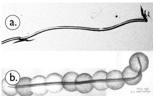
FIG. 1. a.) Fredericks track in Polychrome Litho film. Compare with tracks in Section III J and Fig. 6 in Priem, et.al. [6] b.) Urutskoev track. “Typical track” of Urutskoev and co-workers.
